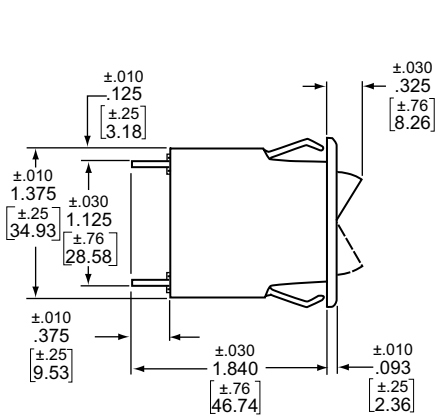
Rocker, Two Pole
