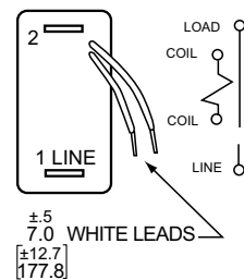
Relay Trip (Note A) Single Pole
