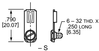
Screw Terminal Adapter (All Versions)
